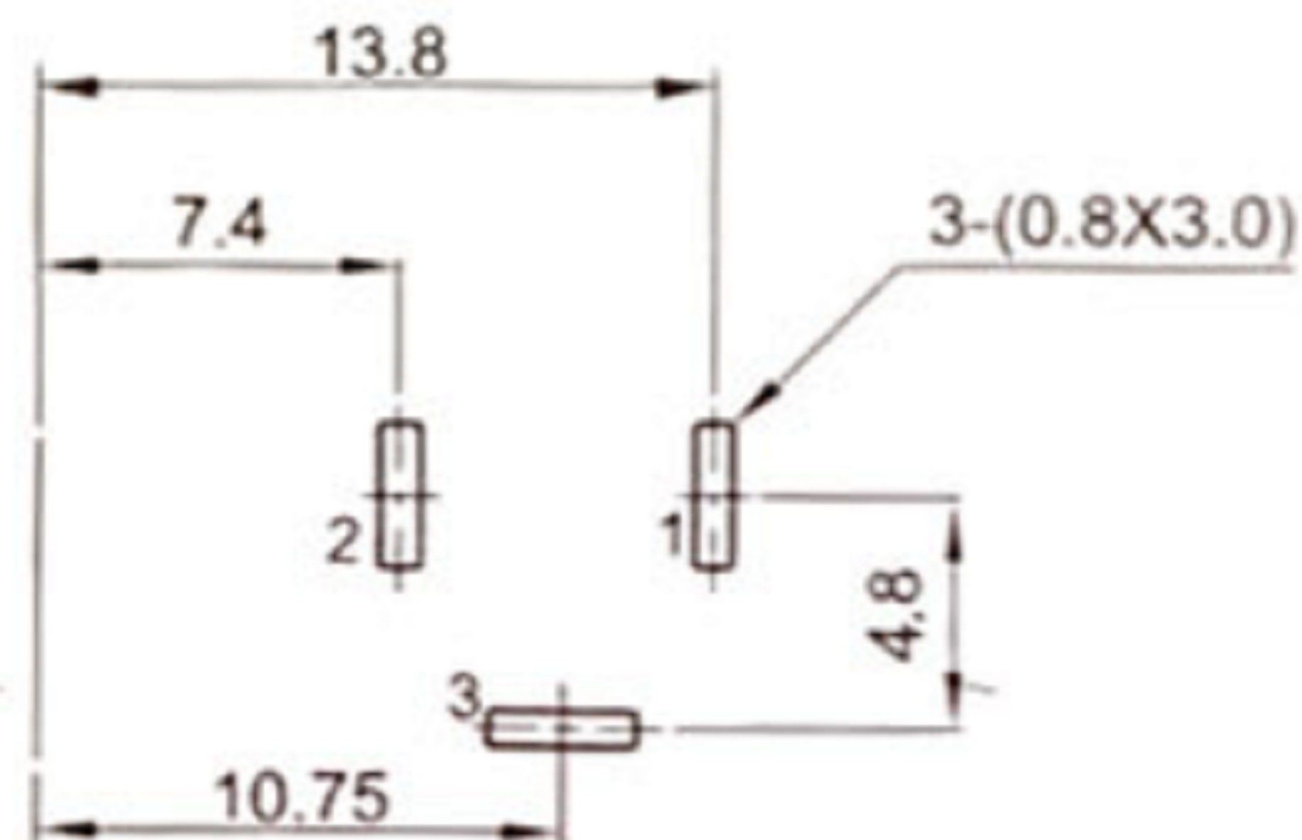
P.C.B LAYOUT TOP VIEW
